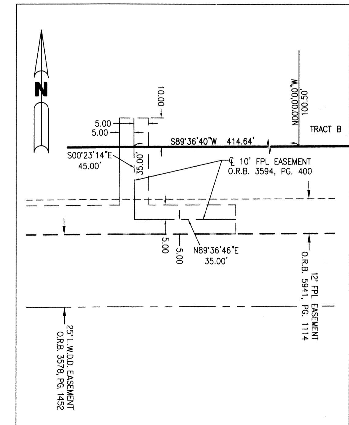
DETAIL "B" SCALE: 1"=20'
