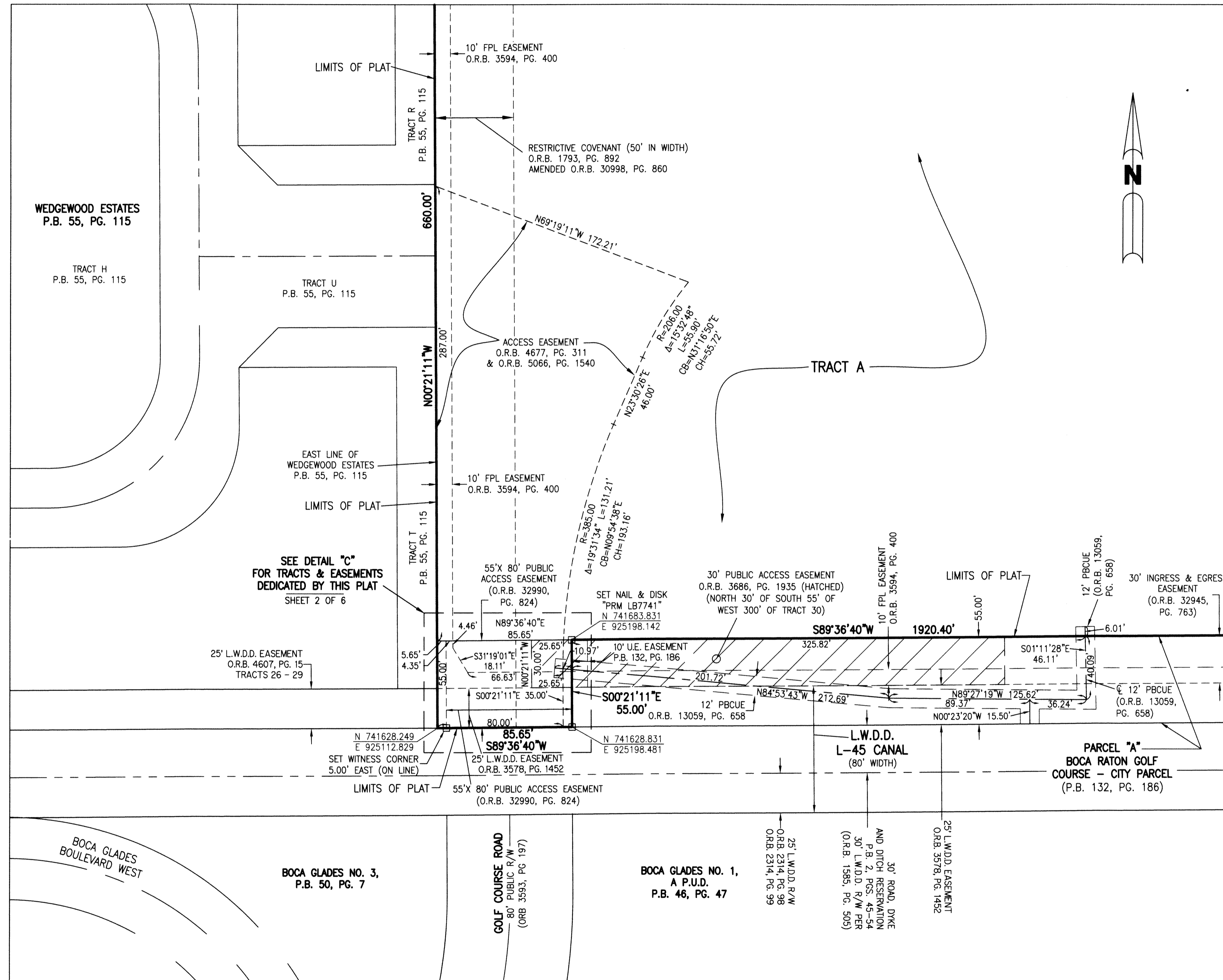
DETAIL "A" (EXISTING EASEMENTS) SCALE: 1"=40'
